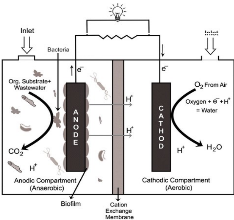
Dual Chamber Microbial Fuel Cell
